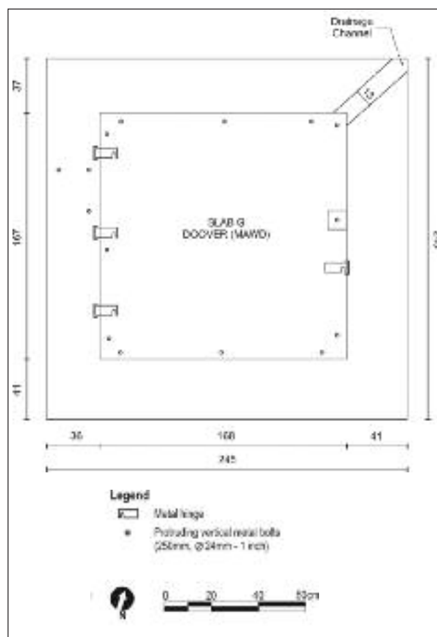
Figure 6: Scale plan of Concrete Slab G.
